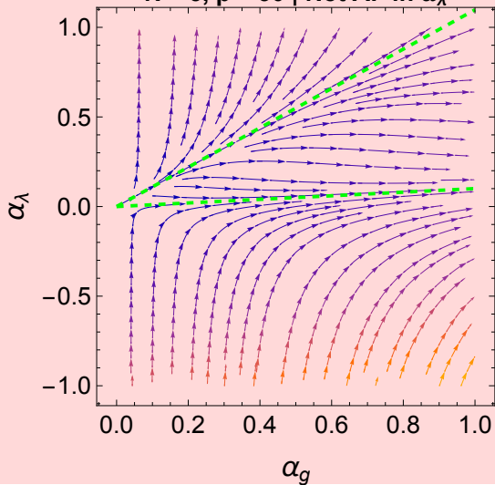
N = 10, p = 30 | AF in \alpha_\lambda
