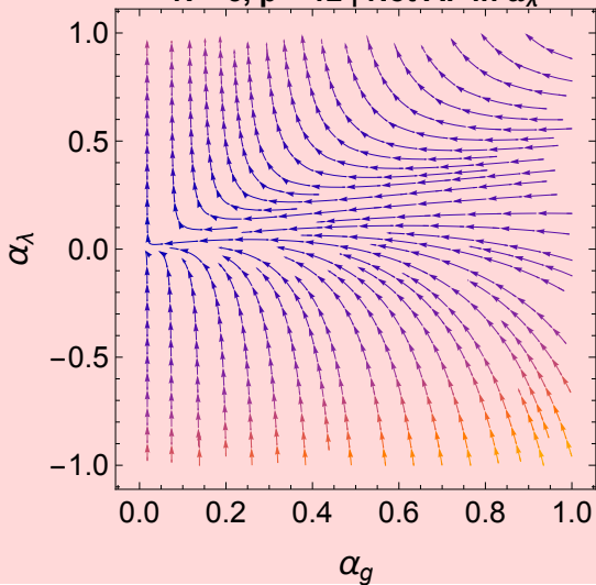
N = 10, p = 12 | Not AF in \alpha_\lambda
